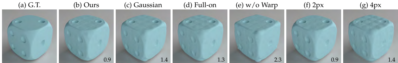
Fig. 12: Impact of lighting patterns, warping and camera pose errors over geometric reconstruction. From the left to right: the ground-truth, the reconstruction using our network, ours with 5 Gaussian noise lighting patterns, ours with a full-on pattern, ours without the warping step and ours with perturbed camera poses (average reprojection error = 2px/4px). Quantitative errors in Chamfer distance are reported in the bottom right corner.
